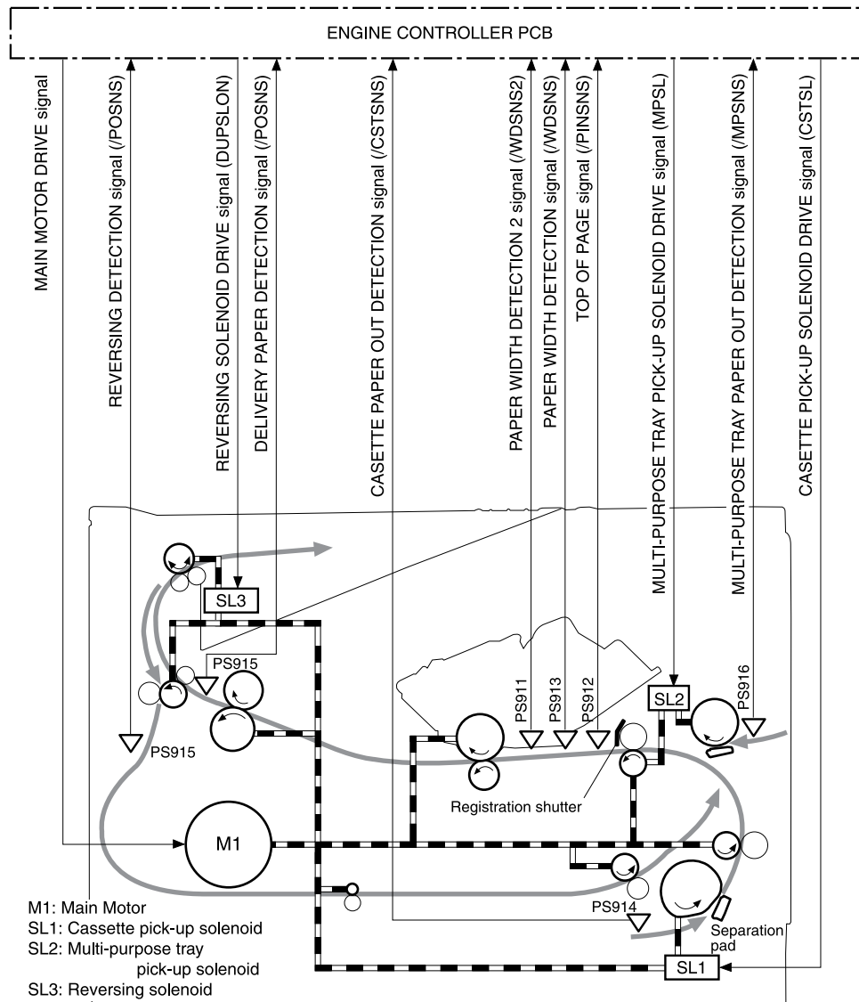
Figure 5-6 Pickup/feed/delivery system
