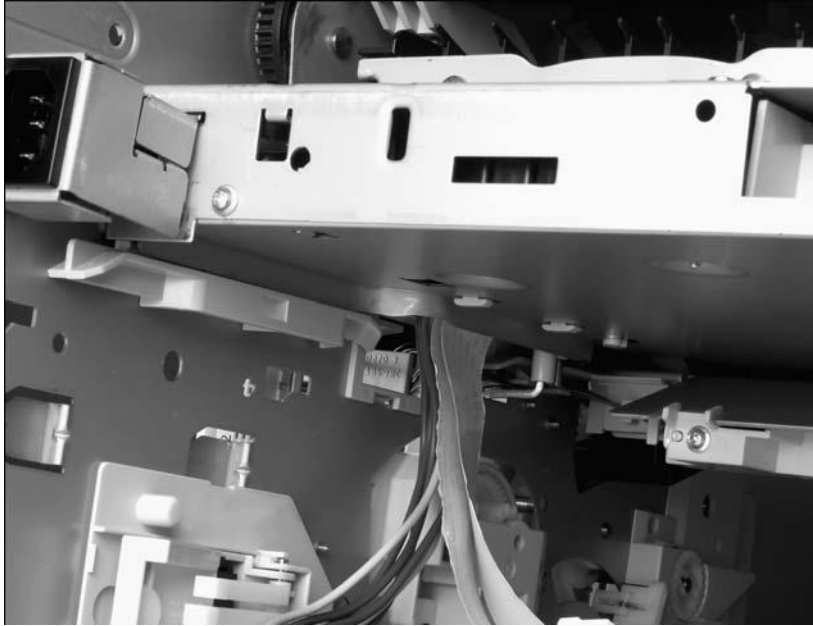
Figure 6-64 Power-supply assembly (6 of 7)
