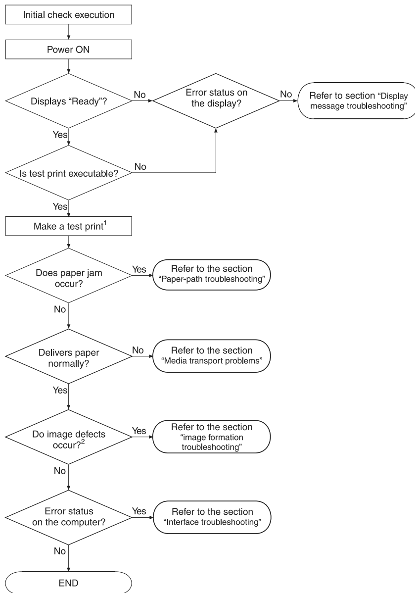
Figure 7-1 Troubleshooting flowchart
