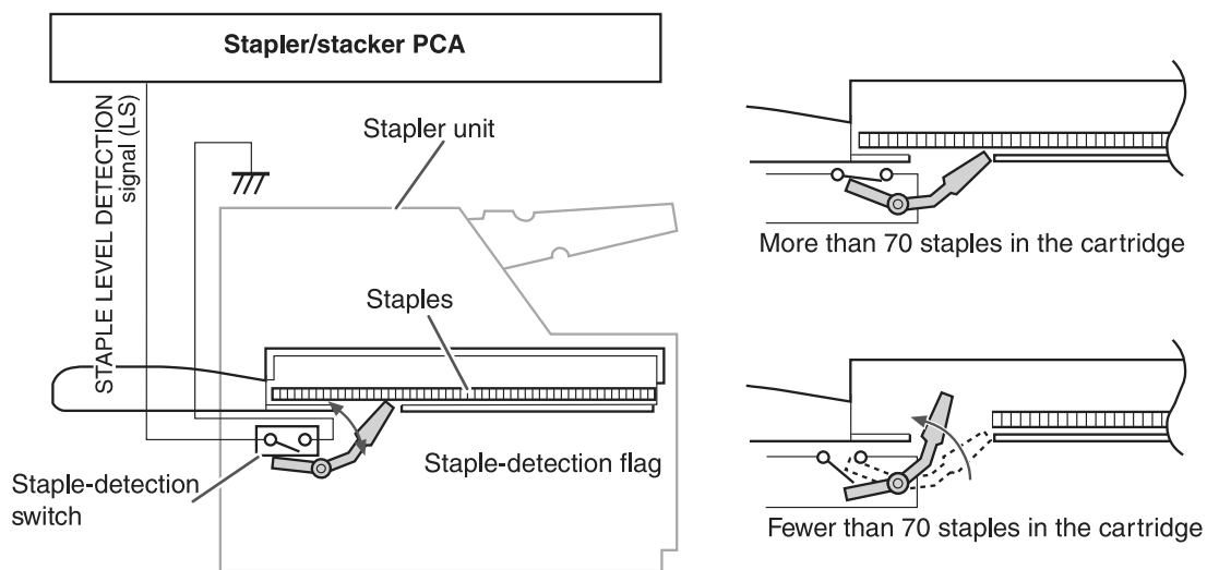
Figure 5-35 Staple-level detection
