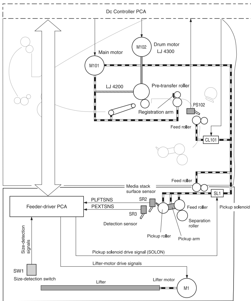
Figure 5-13 1,500-sheet feeder pickup-and-feed diagram
