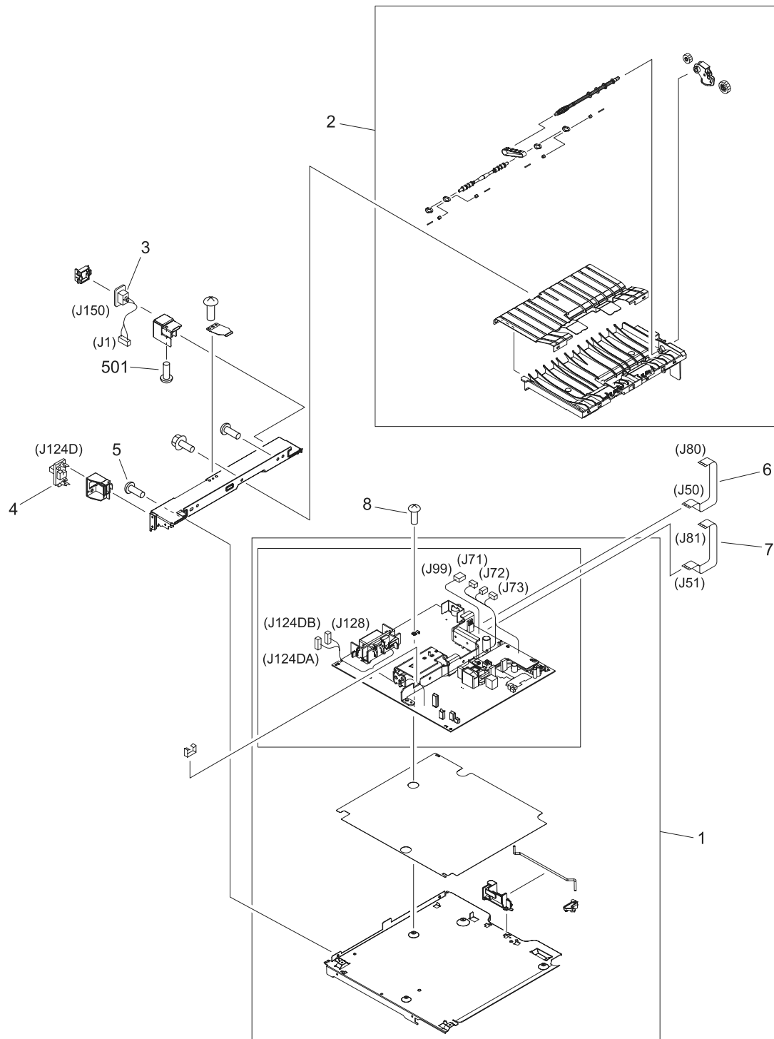
Figure 8-9 Electrical components
