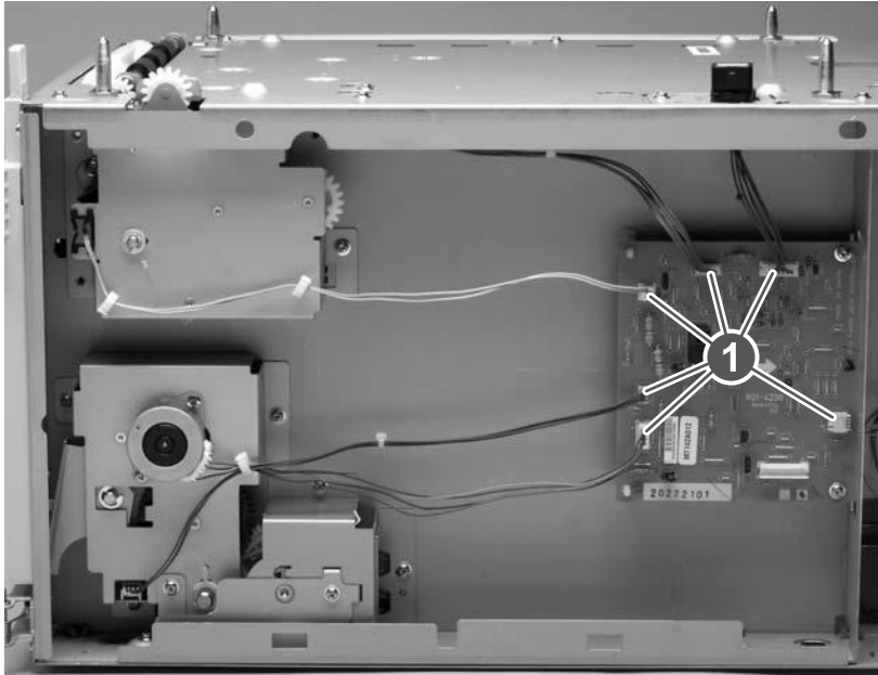
Figure 6-125 1,500-sheet feeder control PCA (1 of 2)
