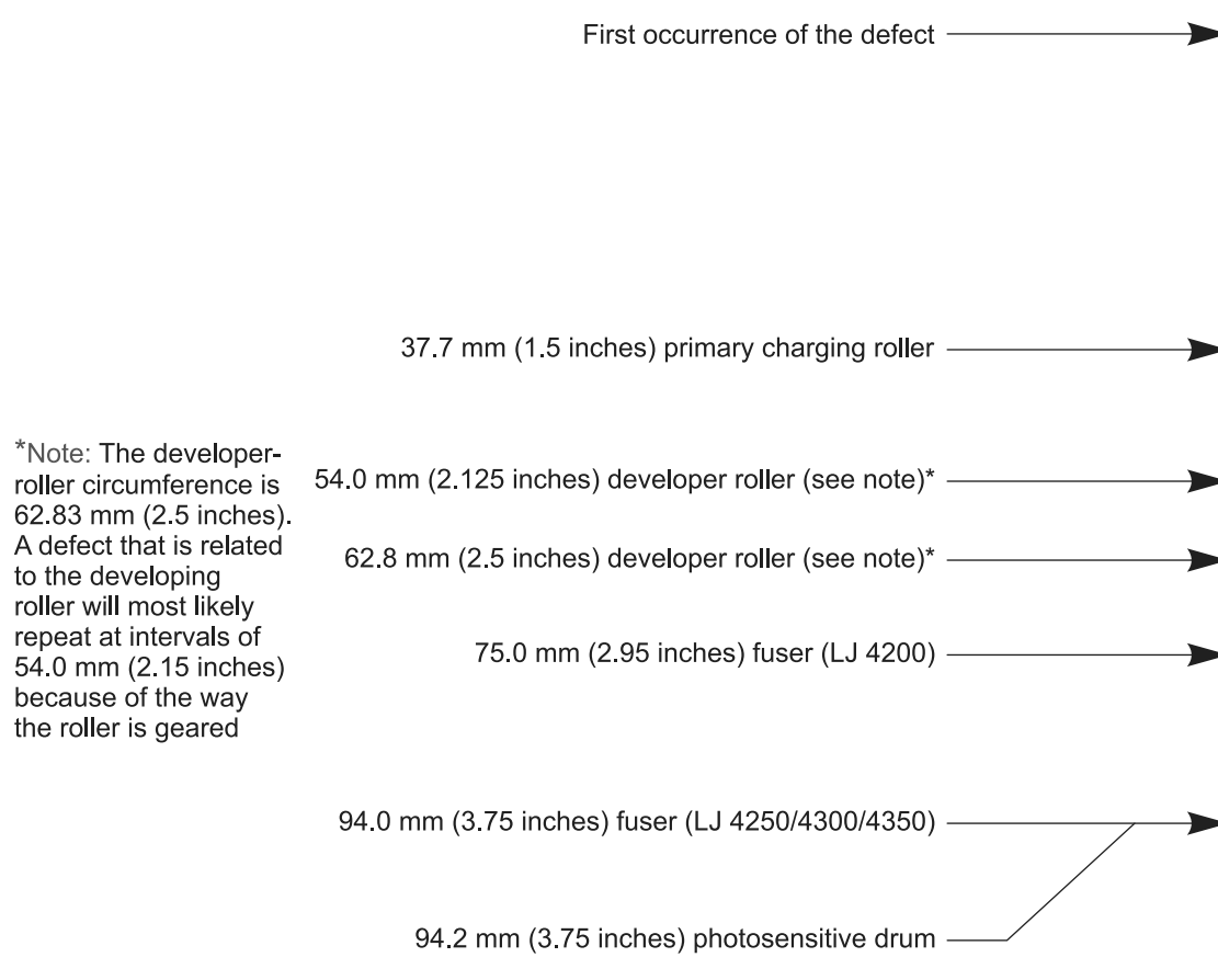
Figure 7-8 Repetitive-defect ruler
