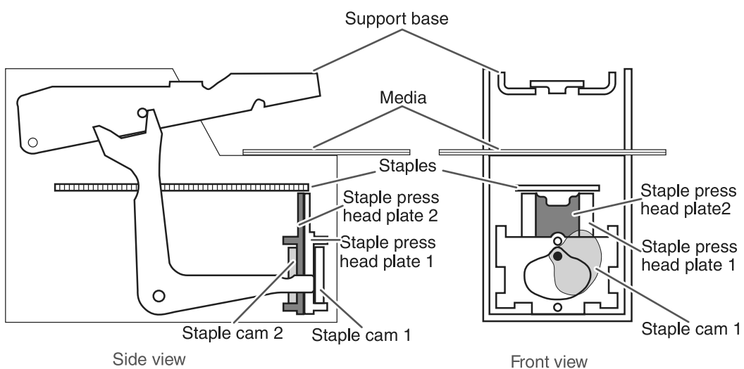
Figure 5-32 Staple operation (1 of 3)
