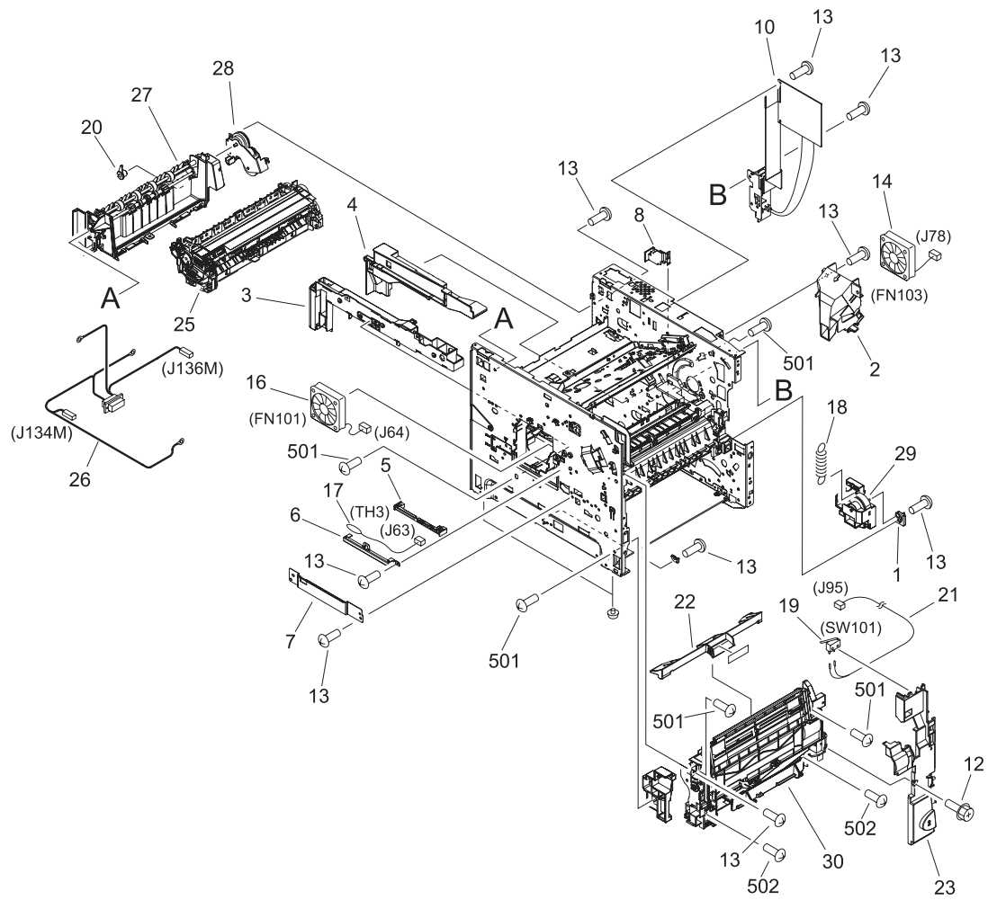
Figure 8-8 Internal components (3 of 3)
