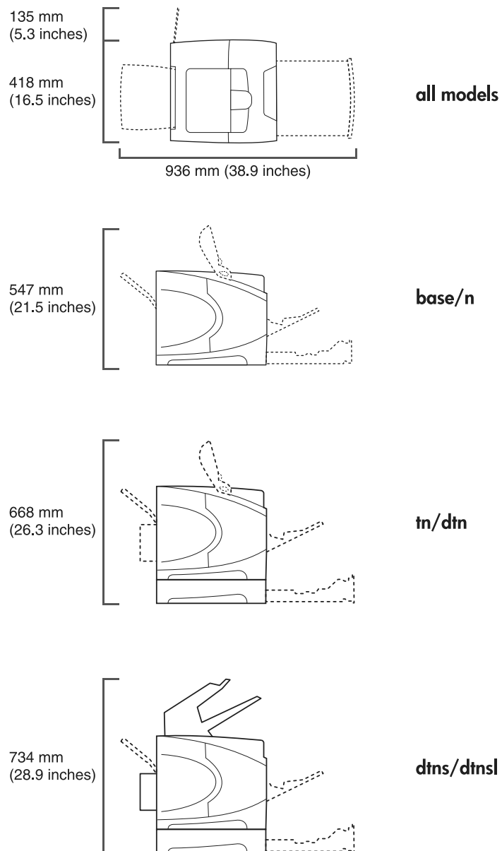
Figure 2-1 Printer measurements
