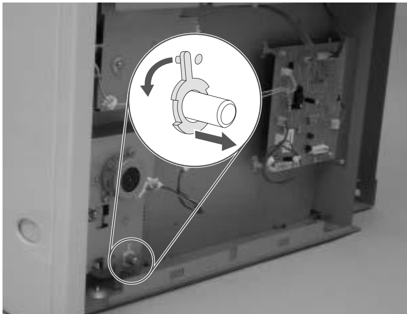
Figure 6-130 1,500-sheet feeder lifter-drive assembly (3 of 4)
