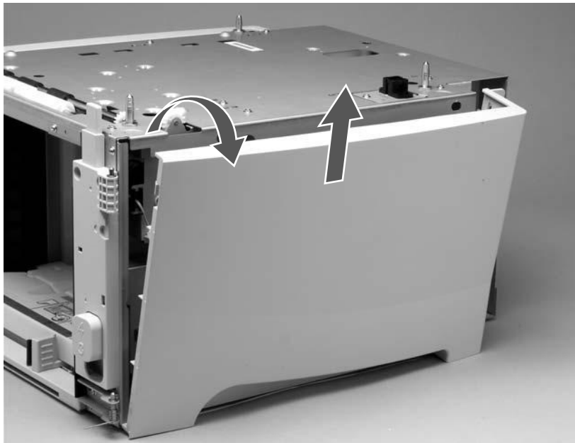
Figure 6-124 1,500-sheet feeder right-side cover (3 of 3)
