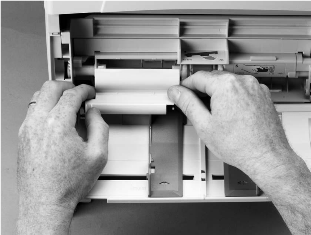
Figure 6-28 Tray 1 (1 of 3)
