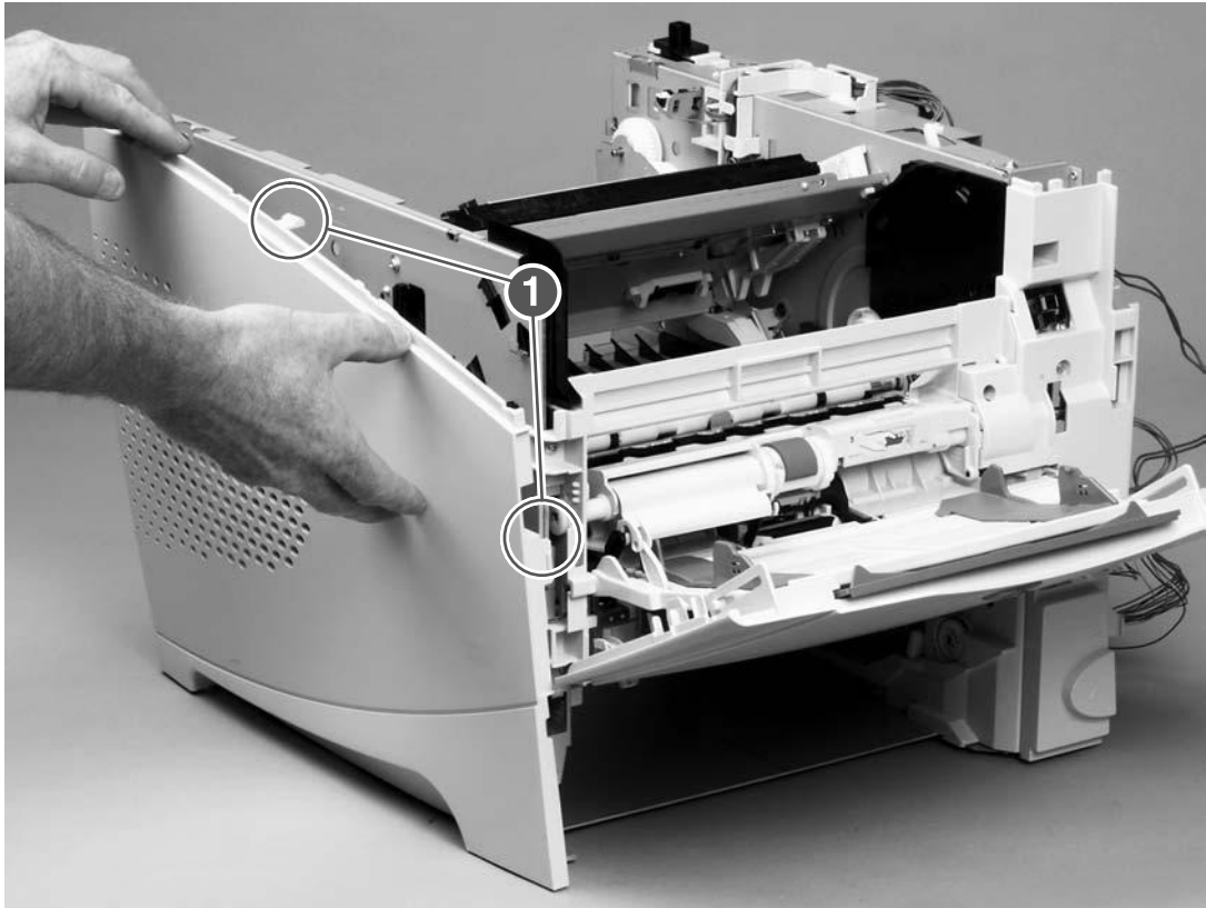
Figure 6-25 Left-side cover
