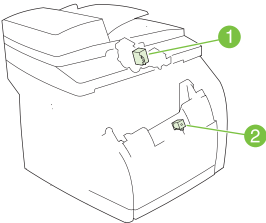
Figure 4-10 Solenoids
