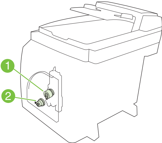
Figure 4-11 Clutches
